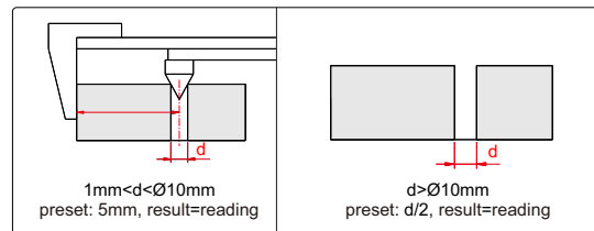
Measure edge to hole center distance
